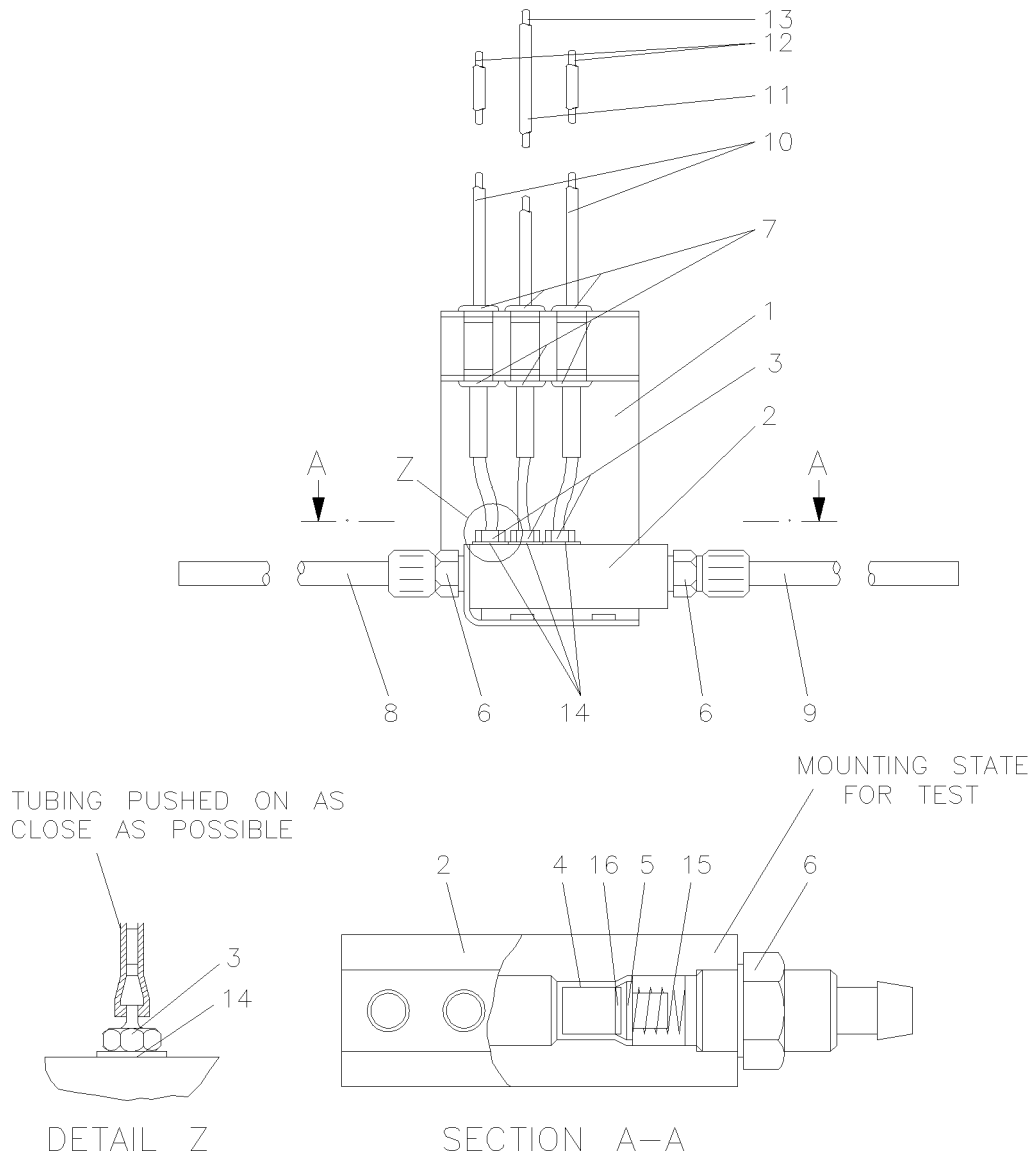
Figure 20-2. Helium Outlet
